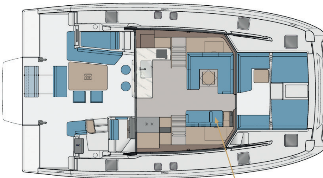
Standard Main Deck
