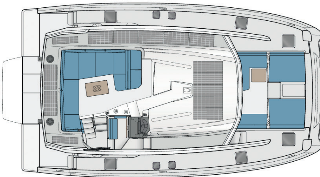
Standard Flybridge
